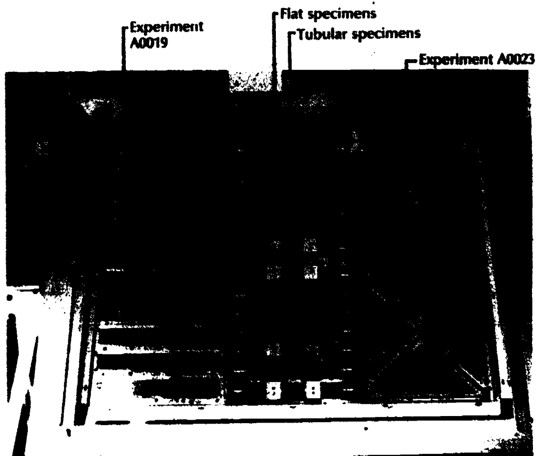
Figure 20.—Polymer matrix composite materials experiment.
