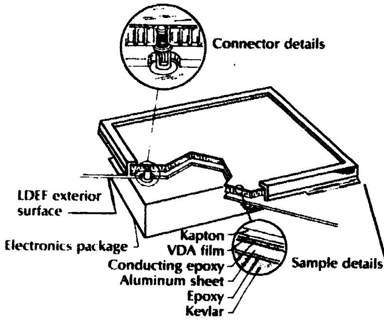
(a) Dielectric sample construction.
