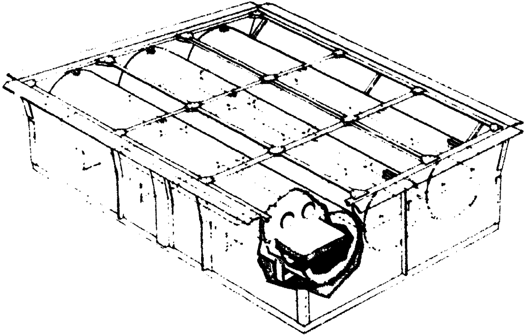
Figure 46. - Cosmic-ray experiment configuration showing location of detector stacks. The light top frame supports the thermal tray cover.
