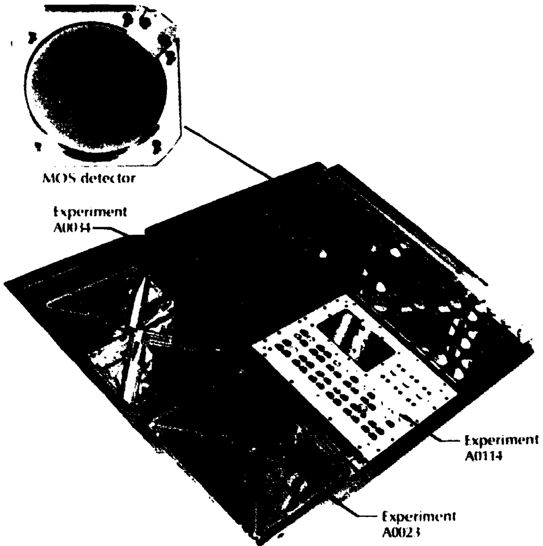
Figure 59 Interplanetary dust experiment.
