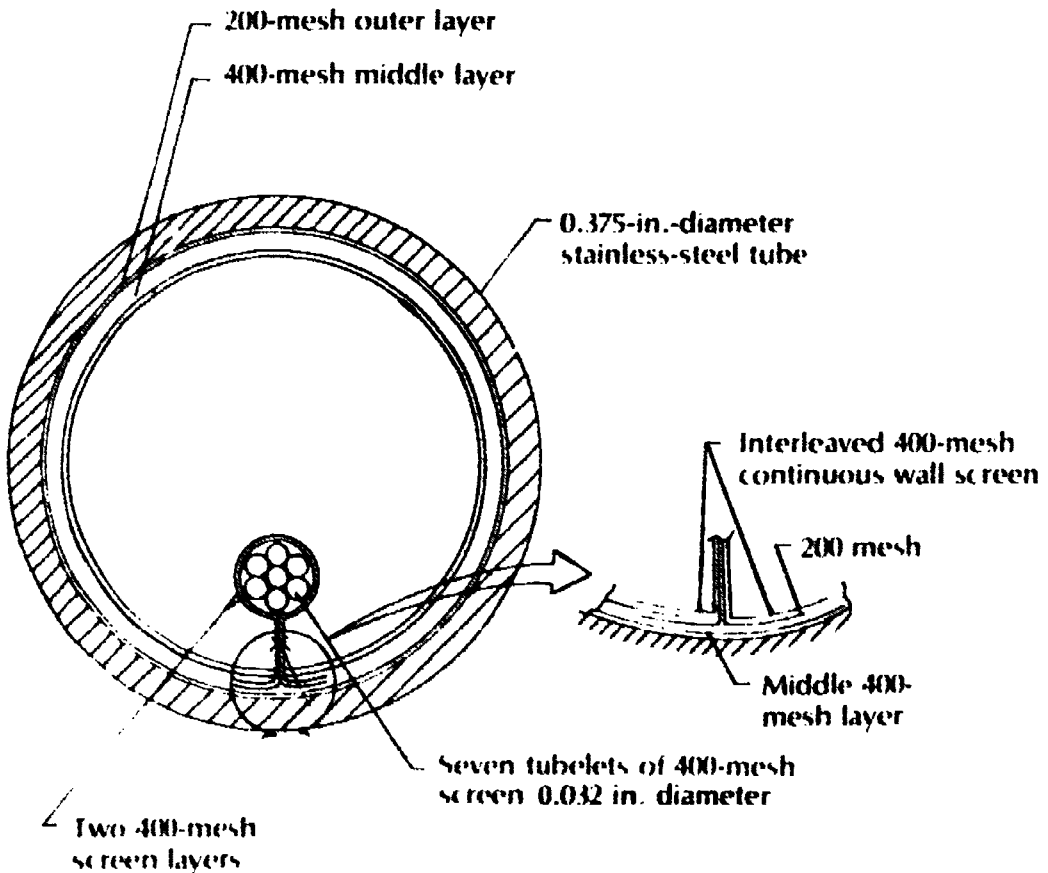
Figure 31. Heat pipe wick design.
