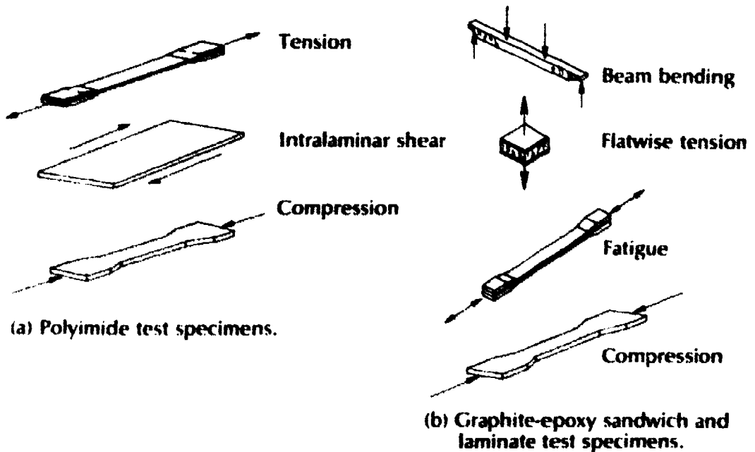
Figure 19.—Graphite-polyimide and graphite-epoxy test specimens.
