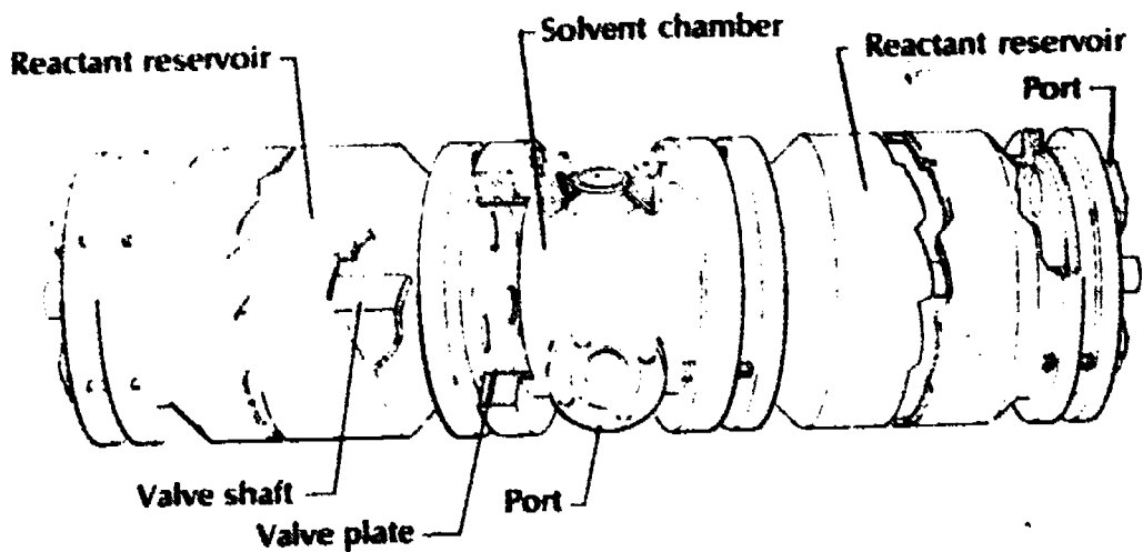
(a) Reactor configuration.
