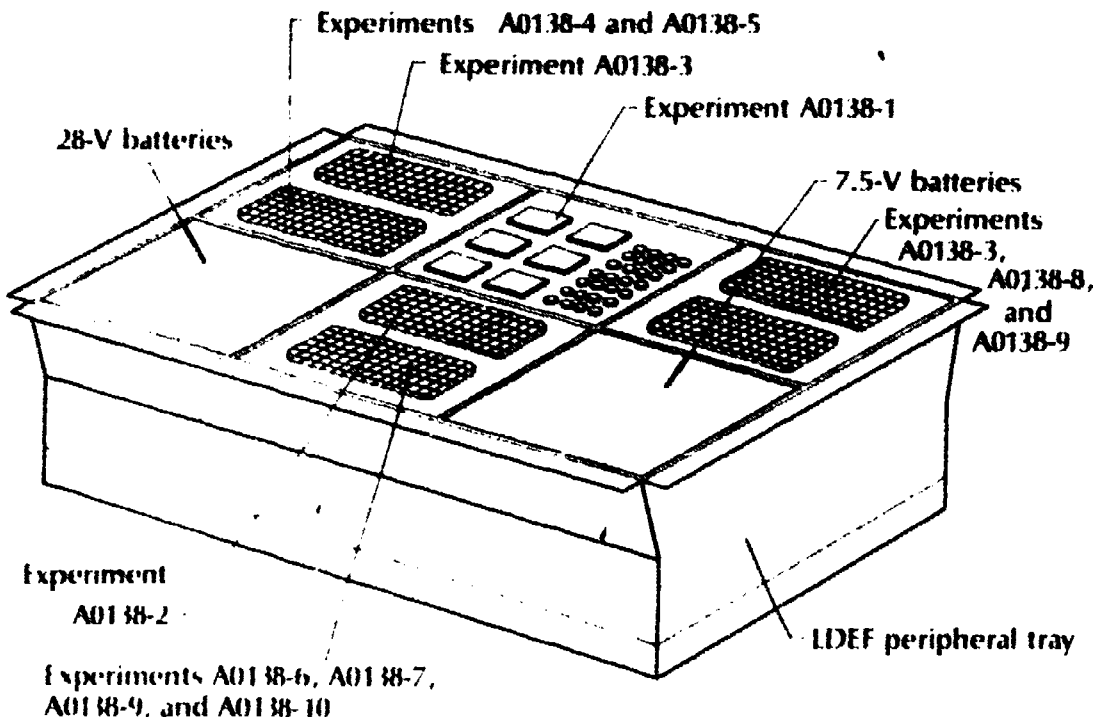
Figure 12.—Layout of French cooperative payload (FRECOPA).
