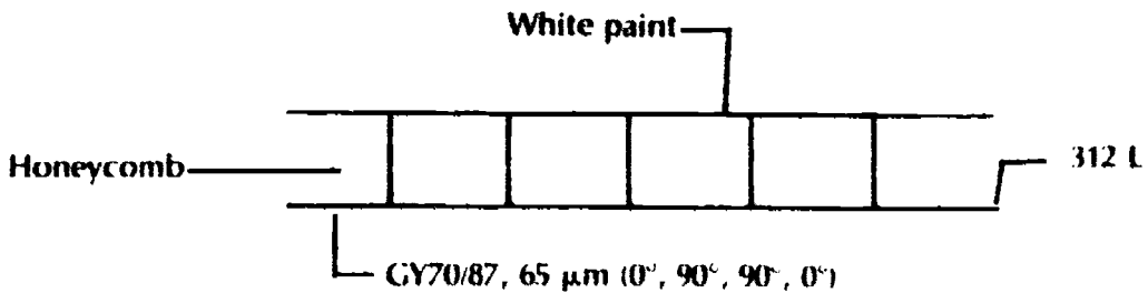
Figure 16.—Structure of sandwich specimen.
