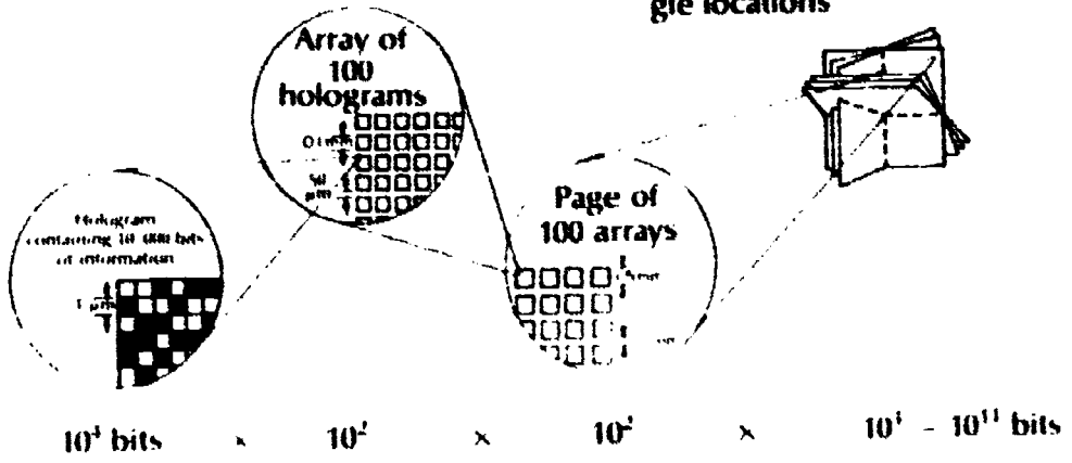
Figure 64. Data storage concept for an optical-phase holographic memory.
