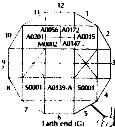
Figure 2.—LDEF experiment integration model.
