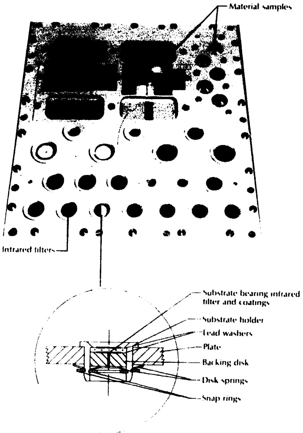
Figure 65 Arrangement of infrared multilayer filter and materials technology experiments.
