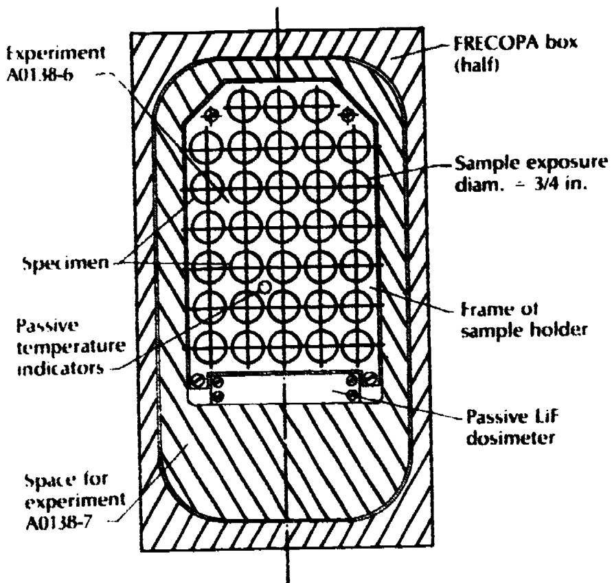
Figure 24.—Layout of thermal control surfaces experiment.
