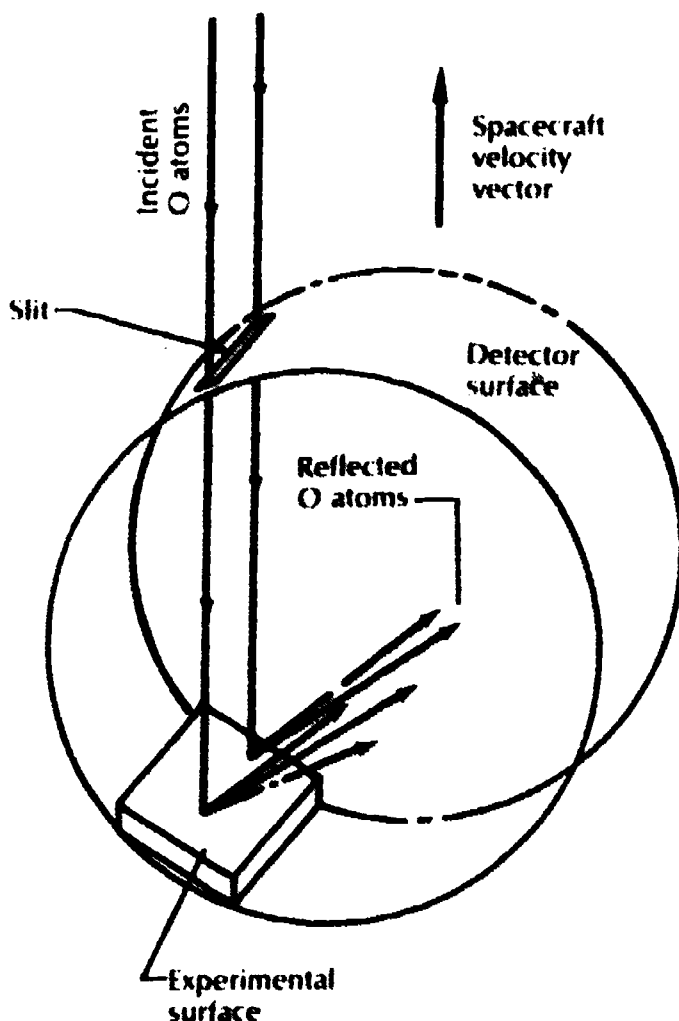
Figure 8.—Cylindrical reflectometer configuration.
