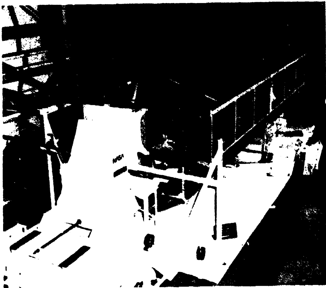
Figure 3 LDEF shown on ground transporter during final checkout before shipment to NASA KSC
