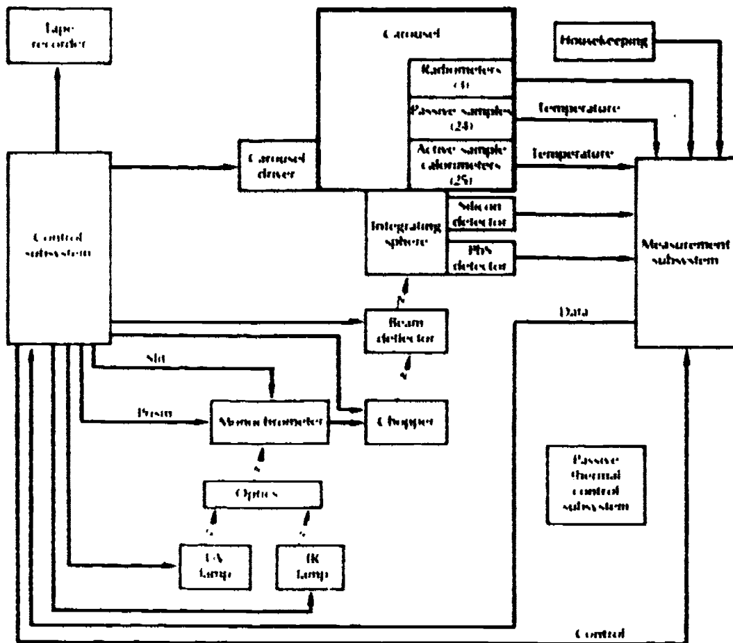
Figure 26. - Simplified block diagram of thermal control surfaces experiment.
