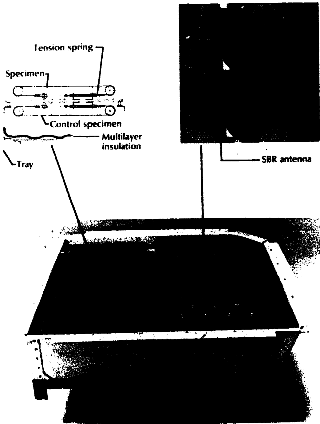
Figure 10.—Space-based radar phased-array antenna experiment.
