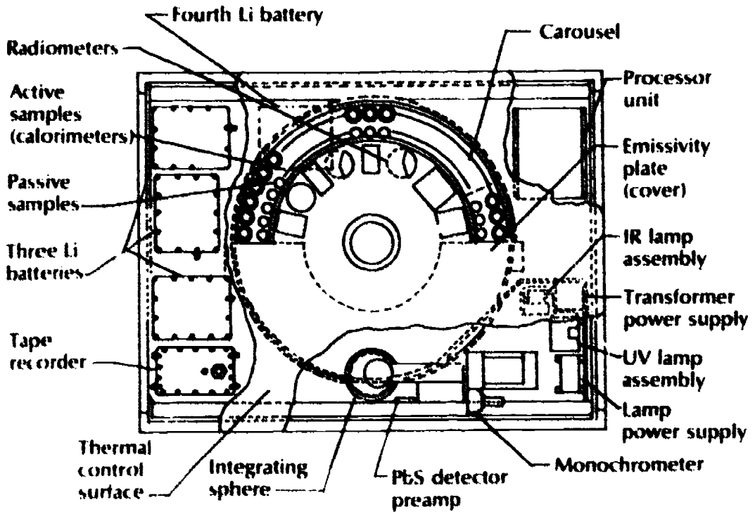
Figure 27. Thermal control surfaces experiment layout showing location of components.
