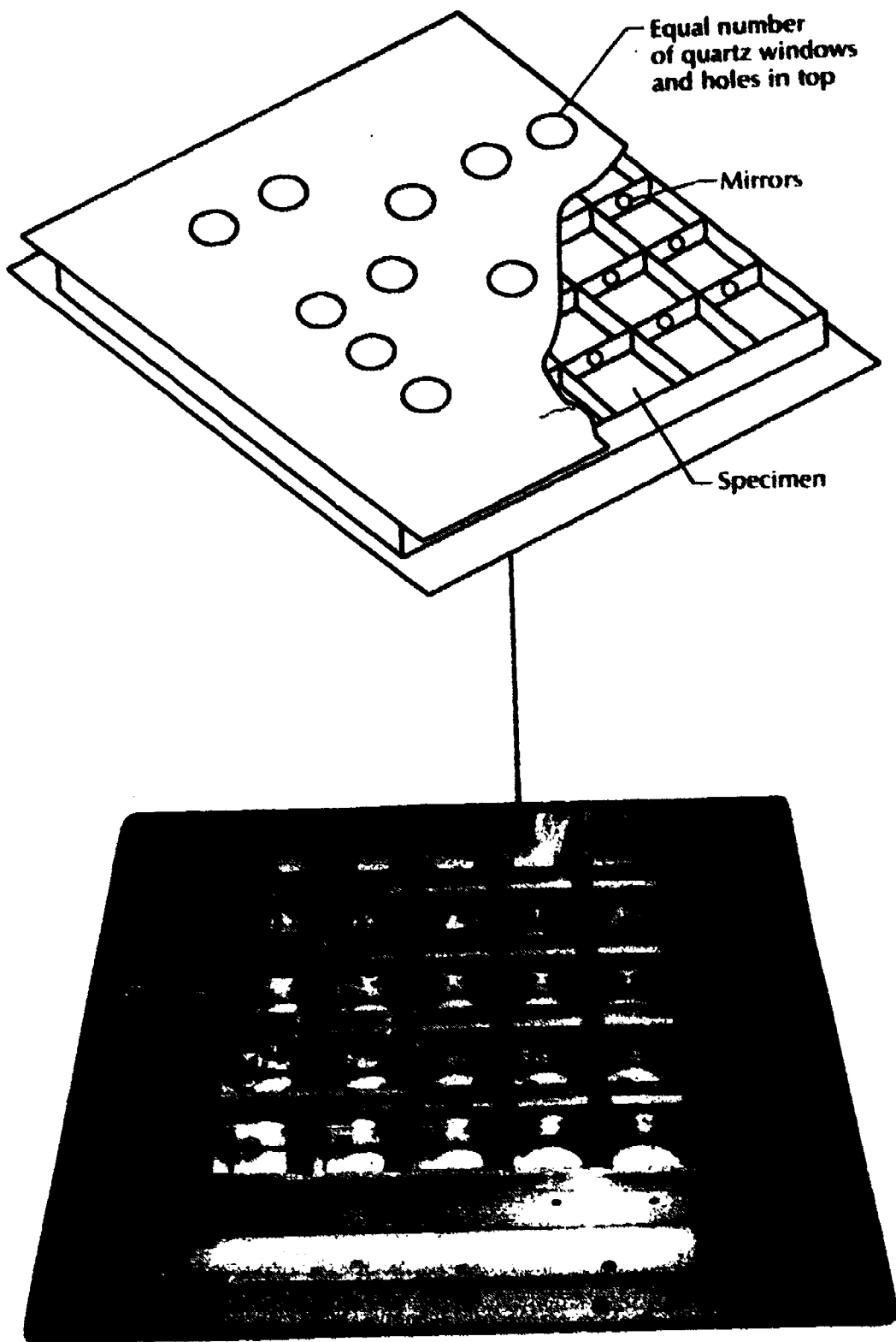
Figure 6.—Atomic-oxygen-stimulated experiment shown with top cover removed.
