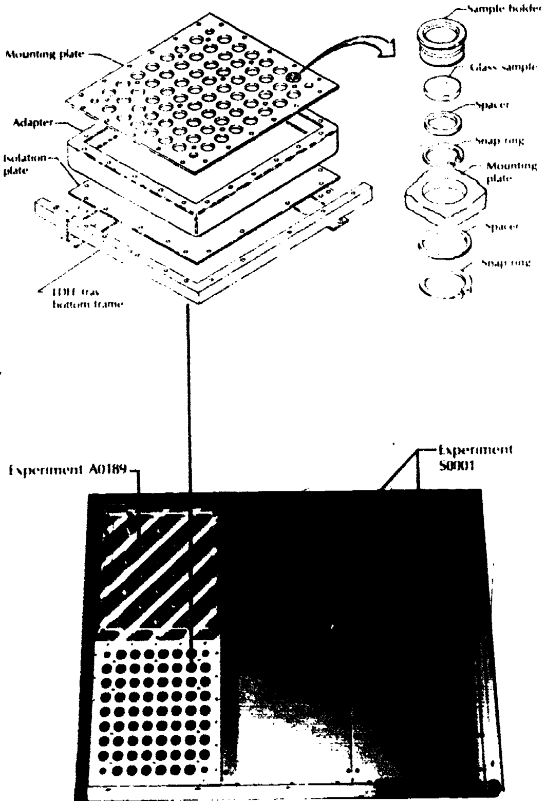
Figure 69. Solar radiation on glasses experiment.
