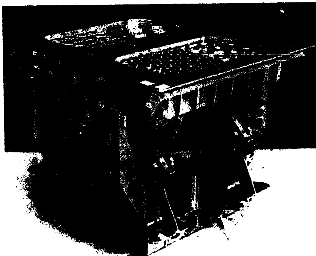
Figure 13.—Photograph of FRECOPA box (open).
