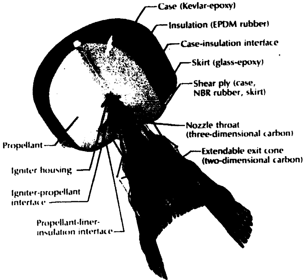
Figure 44. Sketch of IPSM-II motor showing examples of aging samples.
