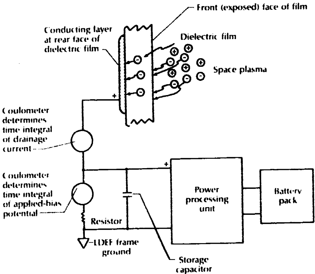
Figure 38. High-voltage drainage experiment concept.
