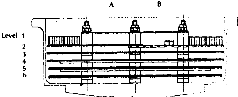
Figure 15.—Section of FRECOPA box showing arrangement of experiment A0138-9.
