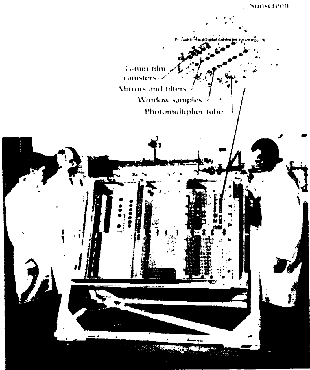
Figure 71. —Active optical system components experiment.
