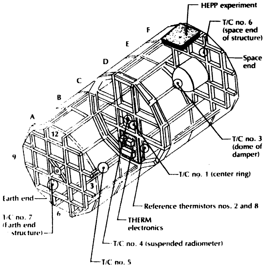
Figure 37. Location of THERM hardware on LDEF.
