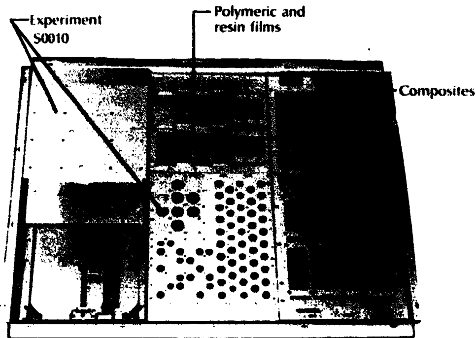
Figure 11.—Space exposure of composite materials experiment shown integrated with Exposure of Spacecraft Coatings experiment (S0010).
