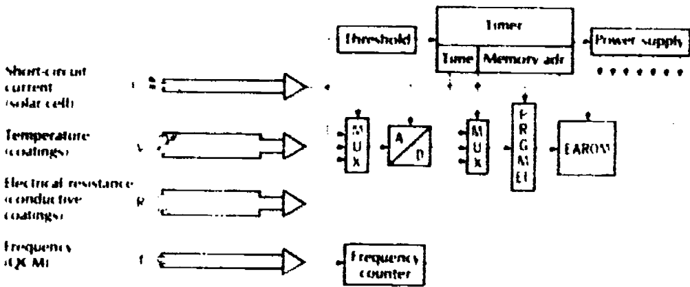
Figure 43. - Electronics block diagram.
