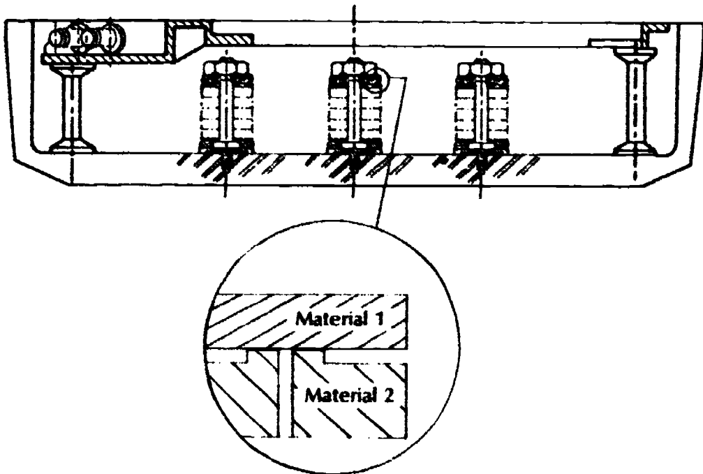
Figure 17.—Layout of the eight washer "spools" within FRECOPA box.
