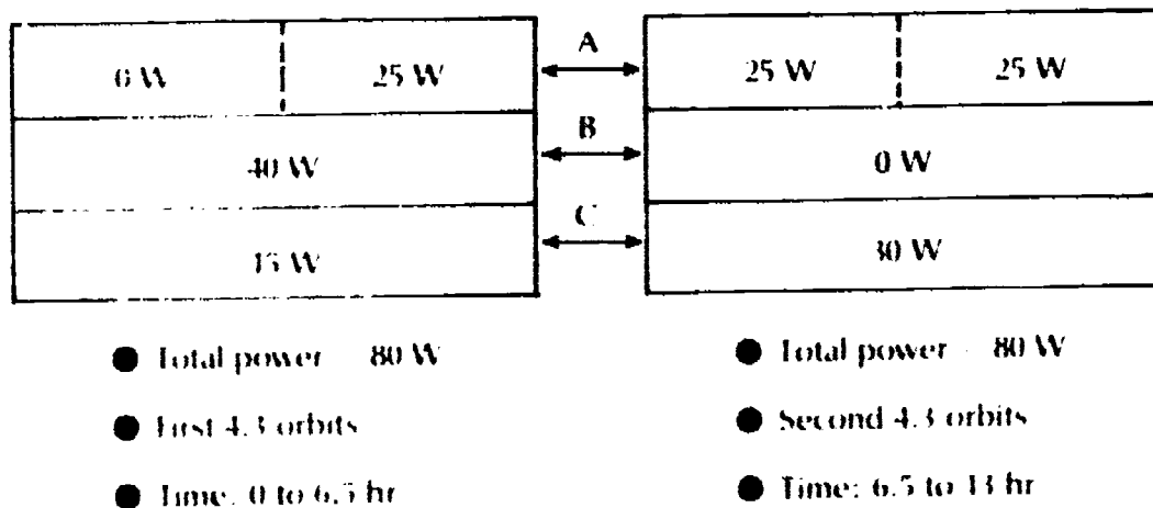
Figure 36. Heating sequence
