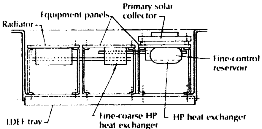
Figure 30. Cascade variable-conductance heat pipe configuration.
