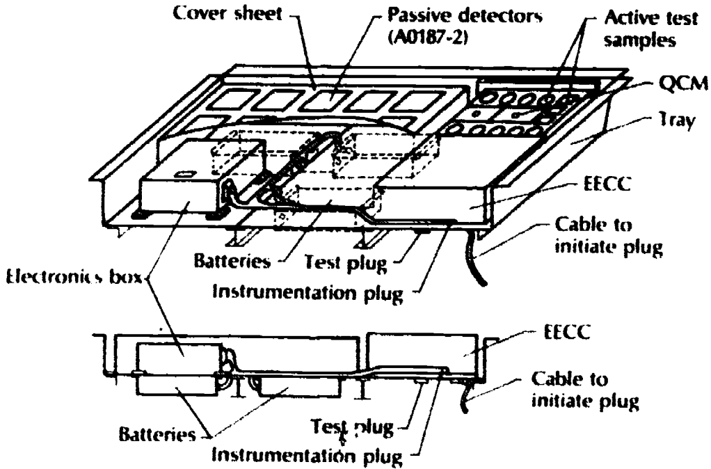
Figure 42. - Experiment arrangement.
