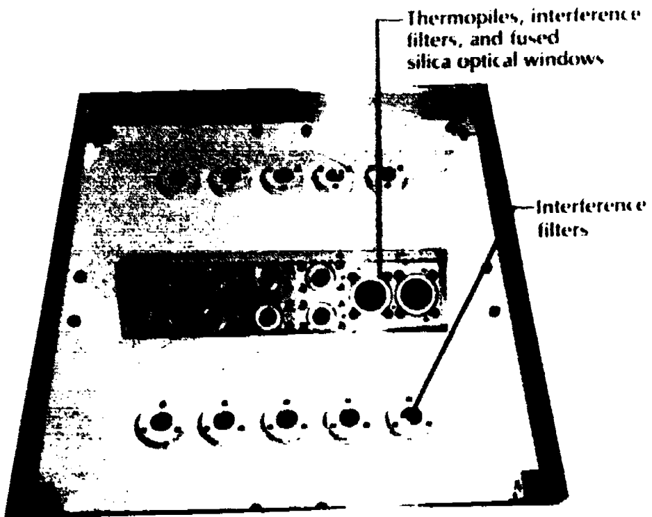
Figure 68.--Solar-channel components.
