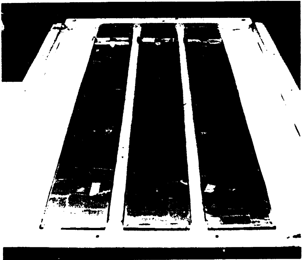
Figure 34.—Transverse flat-plate heat pipe experiment.
