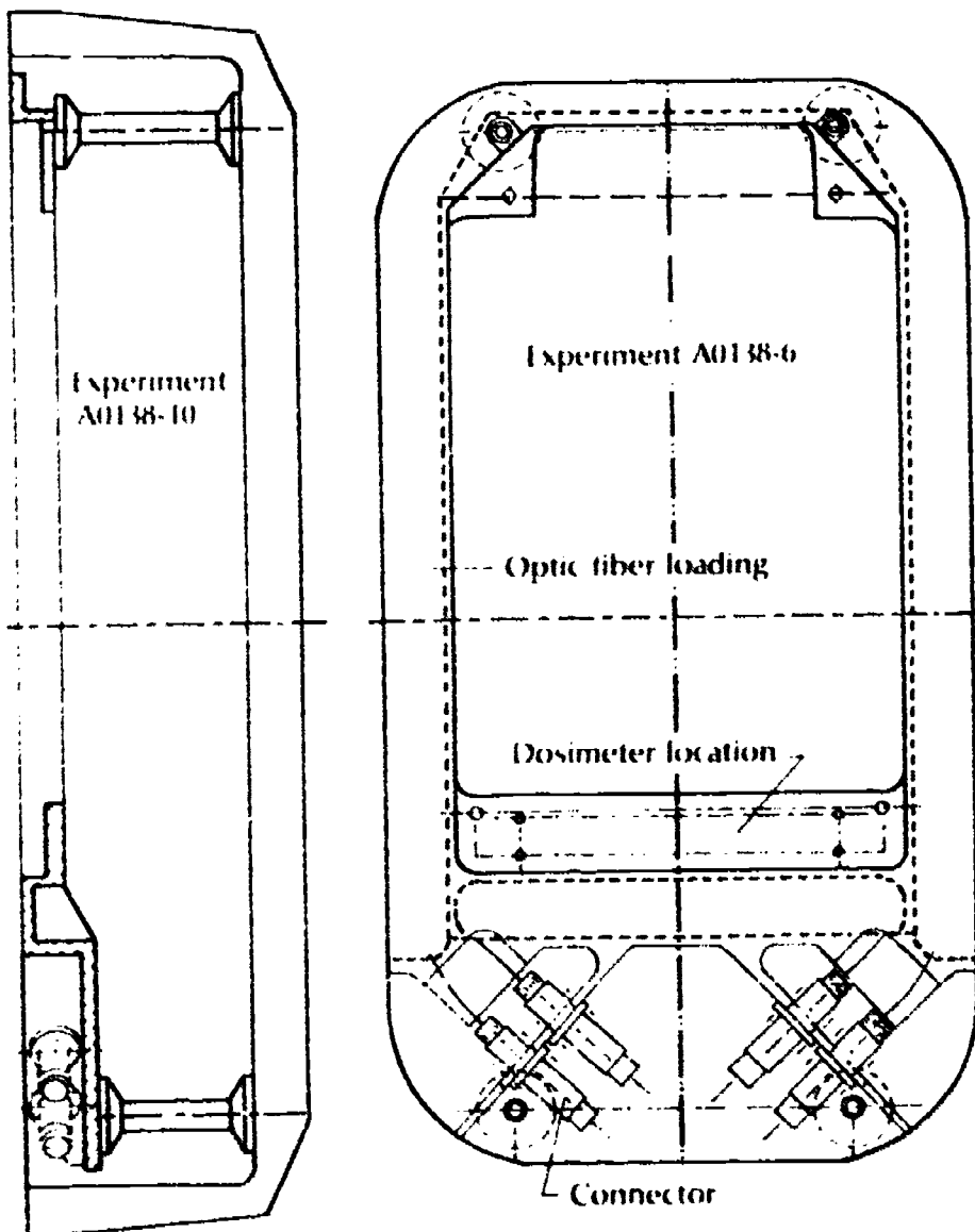
Figure 16. - Optical-fibers experiment configuration.
